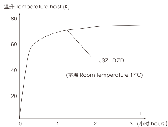
散热器温升曲线 The radiator rising curve
